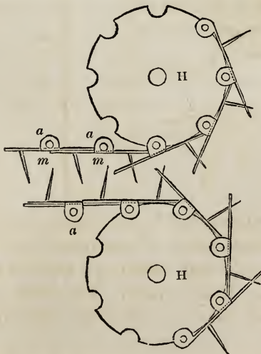
Fig. 25.—Machine for Wool Combing.
