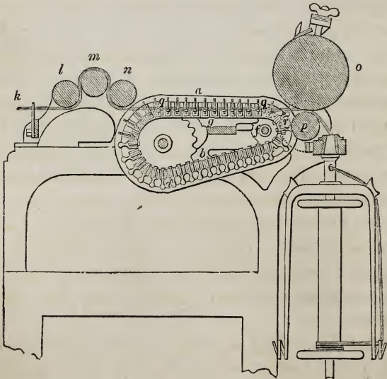
Fig. 40.—Wordsworth's Flax-roving Machine.
