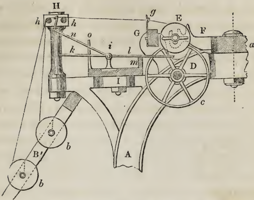
Fig. 49.—Mechanism of Silk Doubling-Mill.—Section.
