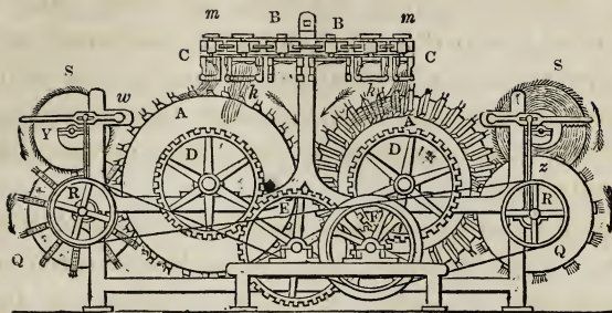
Fig. 39.—Section of Wordsworth's Flax-heckling Machine.
