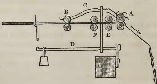
Fig. 29.—Worsted Throstle.
