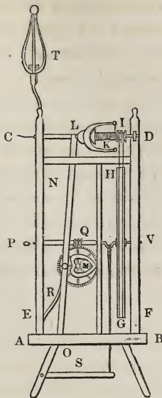
Fig. 44.—Self acting Flax-wheel.
