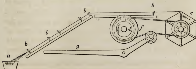
Fig. 46.—Cocoon Filature.—Section of Reel.
