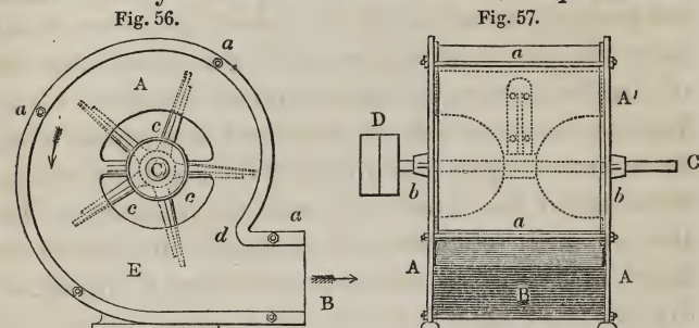
Fig. 56.—Side View of the Ventilating Fan.
