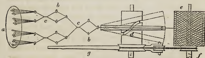
Fig. 45.—Cocoon Filature.—Plan of Reel.
