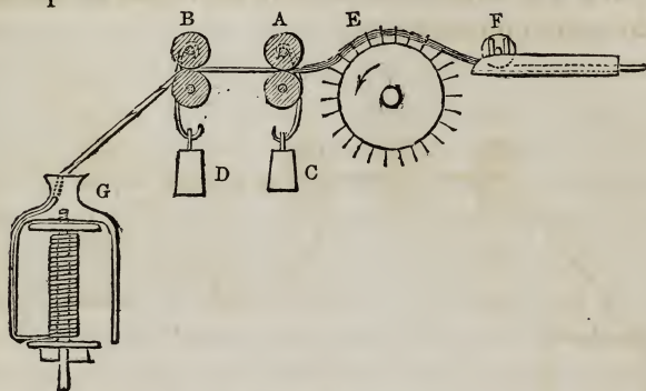
Fig. 27.—Worsted Roving.
