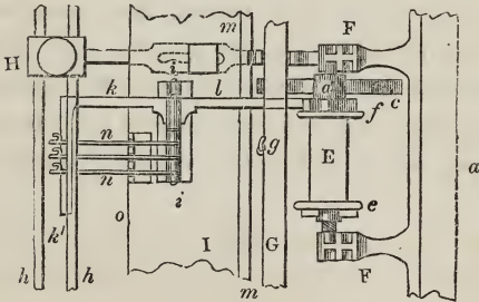
Fig. 50.—Mechanism of Silk Doubling-Mill.—Plan.
