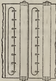
Fig. 26.—Hinge-pieces.
