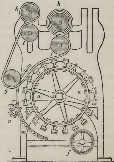
Fig. 35.—Atkinson's and Walker's Gig Mills united.
