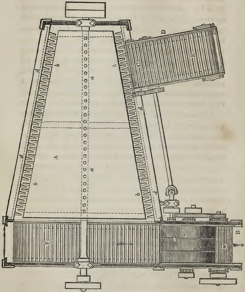
Fig. 30.—Lilly's Conical Willow.
