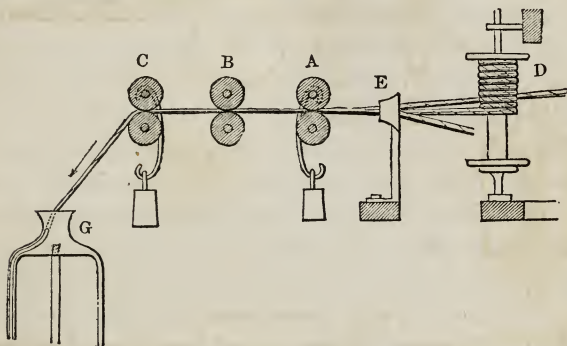
Fig. 28.—Worsted Spinning.
