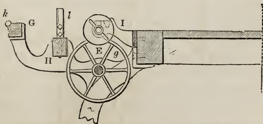
Fig. 48.—Bobbin Mechanism of the Silk Engine.
