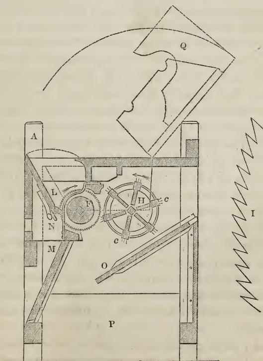
Fig. 17.—Whitney's Saw-gin.
