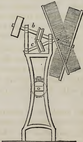
Fig. 23.—Platt's Wool-Combing Machine.
