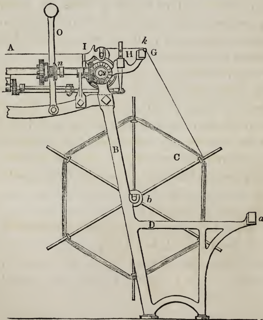
Fig. 47.—Silk-Engine, or Swift.
