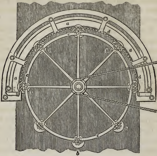
Fig. 37.—Oldland's Cloth Shearing Machine.
