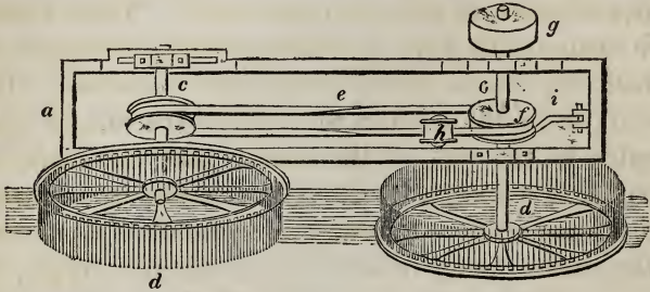
Fig. 22.—Platt's Wool-Combing Machine.
