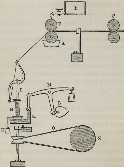
Fig. 43.—Wet Flax Spinning.
