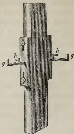
Fig. 21.—Comb Post.
