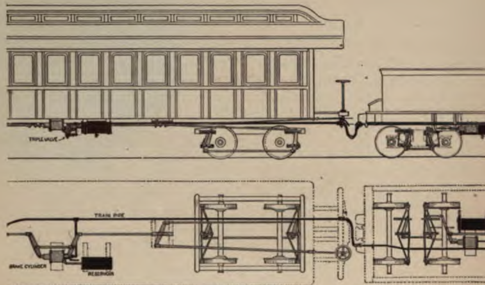
Plan and Elevation of Air-brake Apparatus.—Reset-
