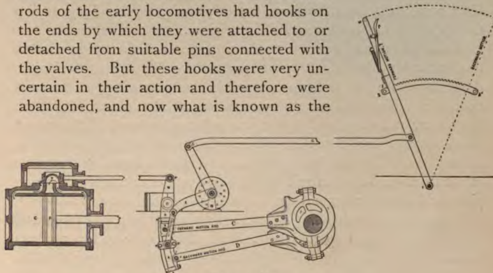
Fig. 24.—Valve Gear.
