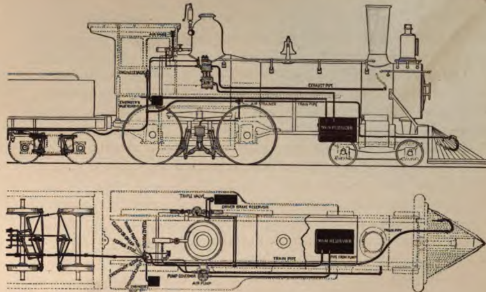
Reservoirs and piping in solid black; brake gear shaded.
