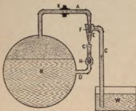
Fig. 18.—Rudimentary Injector.
