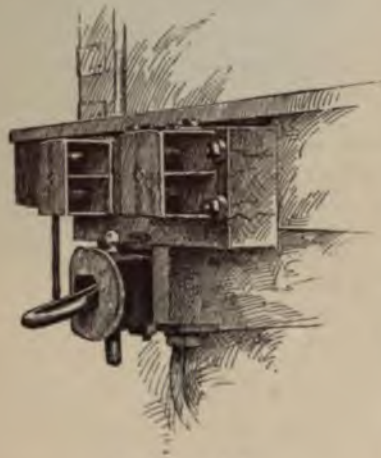
Link-and-pin Coupler.
