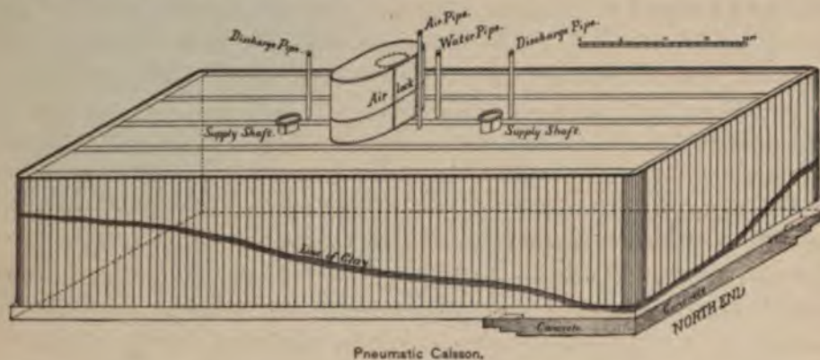
Pneumatic Caisson.
