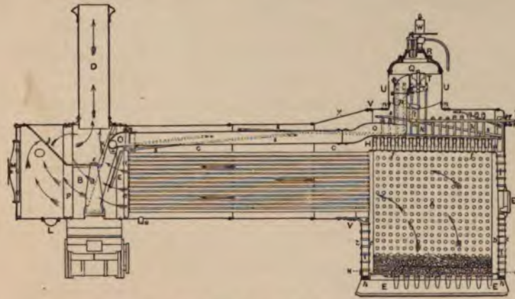
Fig. 16.—Longitudinal Section of a Locomotive Boiler.
